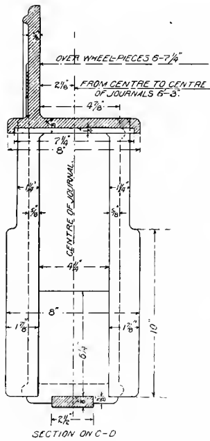
Fig. 5480. Cross Section.
